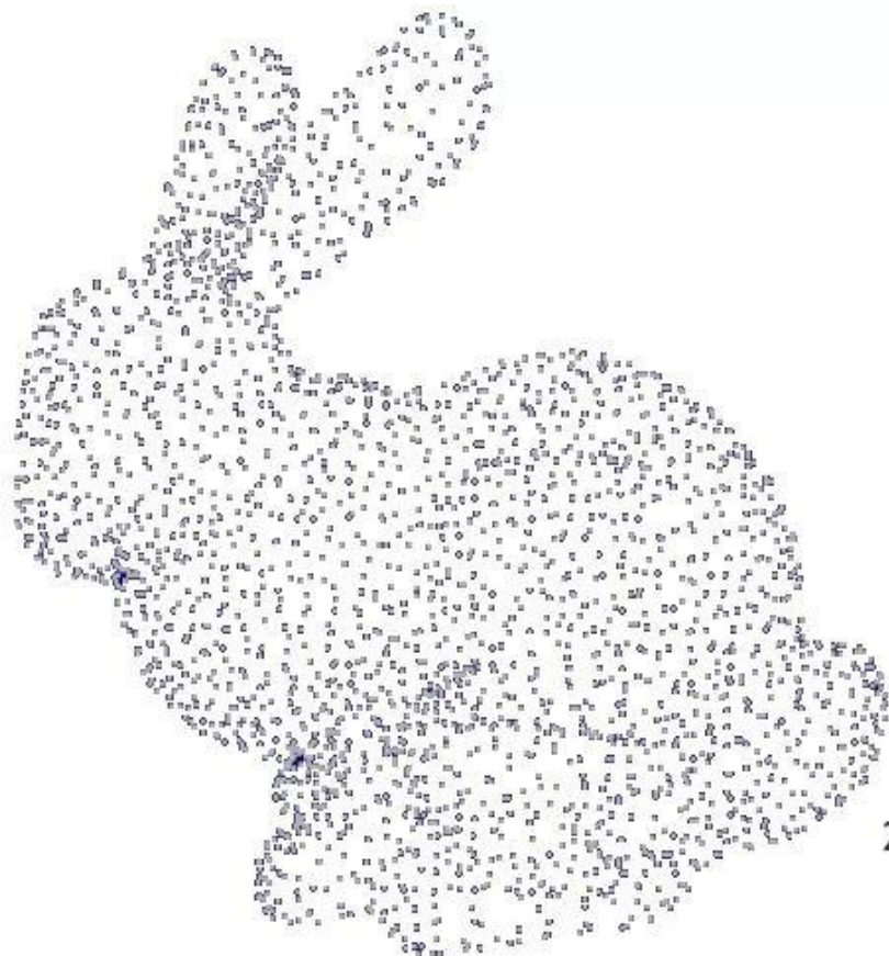
Point Cloud
