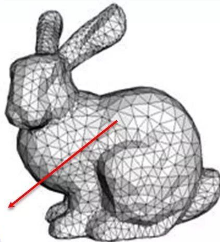
Mesh (shaded)
